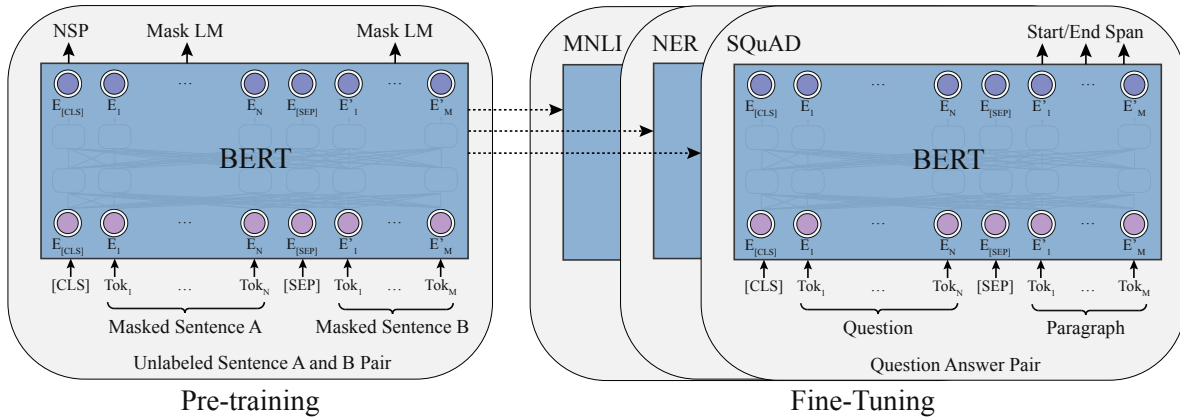
Figure 7: The pre-training and fine-tuning phases for BERT.
